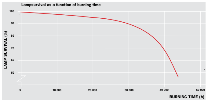
The 12 h-switching cycle is defined as the time when 10% of the lamps in an installation are failed. The lumen depreciation at this time is indicated with approximately 15%.
