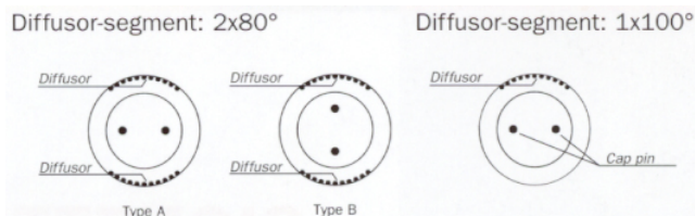
Light distribution effect of Signette-LL-D in a double sided sign
