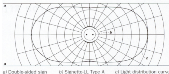
Light distribution effect of Signette-LL-D in a double sided sign
